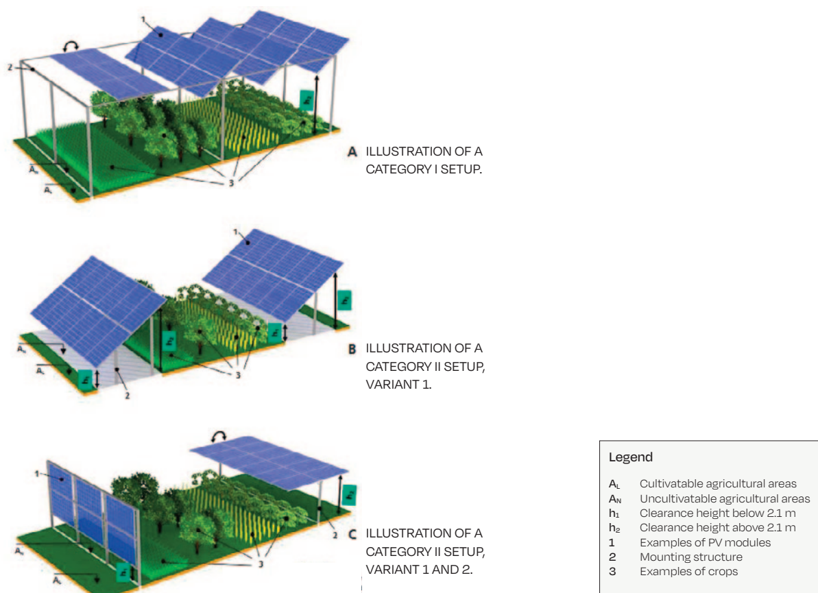
FIGURE 7 DIFFERENT TYPES OF AGRI-PV INSTALLATIONS
